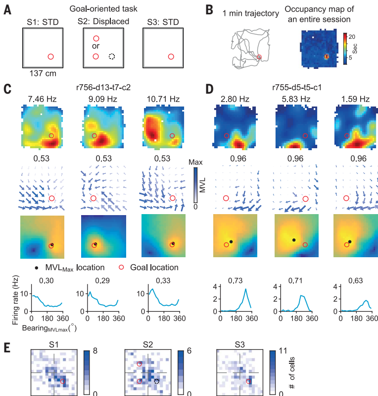
Fig. 3. LEC cells show goal-related egocentric tuning. (A) The goal-oriented task. A single food well (red circle) was shifted from the standard goal location (STD) in session 1 to one of two displaced locations in session 2, and then back to the original standard location in session 3. (B, left) Typical trajectory of rats in this task for 1 min. (Right) Typical occupancy map in an entire session. The goal location is overoccupied. (C) An example cell in three sessions (columns). (Top to bottom) Spatial rate maps, head direction tuning field plots, MVL maps (red circle, food well), and egocentric bearing tuning curves for MVL_{Max} locations. The MVL_{Max} locations for this neuron coincided with the current goal location in each session, as shown in the MVL maps. (D) Another example cell. The standard goal location was represented on the MVL maps regardless of the current goal locations. (E) 2D histograms of the distributions of MVL_{Max} locations in three sessions.
