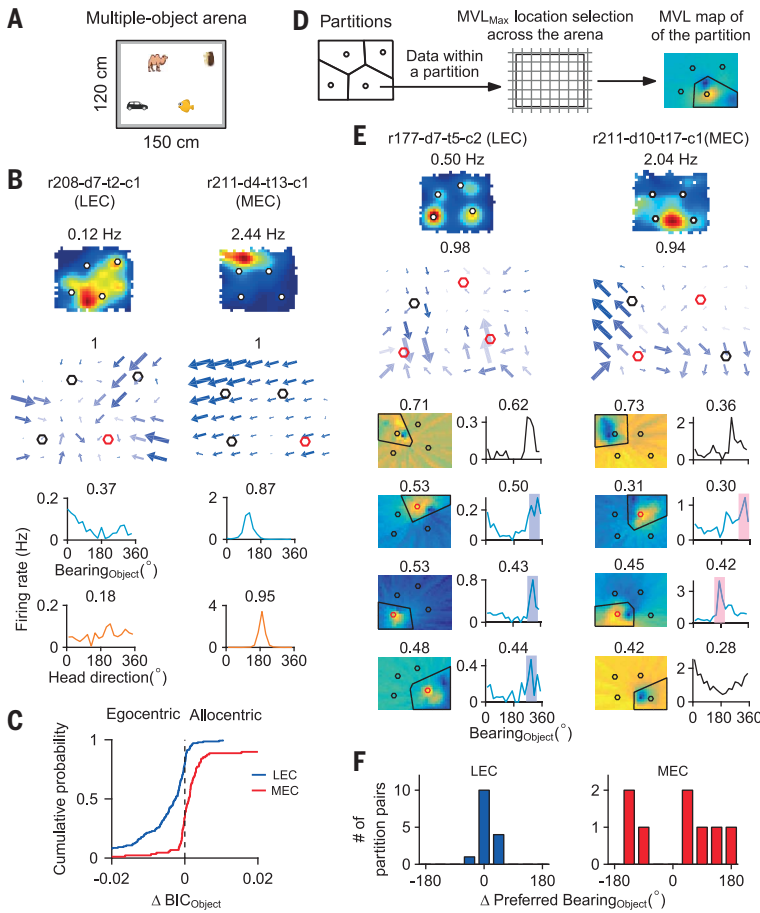
Fig. 2. LEC but not MEC cells show egocentric bearing tuning of 3D objects. (A) The multiple-object arena. (B) Example cells from LEC (left column) and MEC (right column). Top to bottom, spatial rate map (circles denote the objects), head direction tuning field plot (red circle denotes the object with the highest MVL_{Object} ), egocentric bearing tuning curve for the object with the highest MVL_{Object} , head direction tuning curve. (C) Cumulative distributions of best \Delta BIC_{Object} values for LEC and MEC cells. (D) Schematic showing construction of an MVL map with data in a local partition. (E) Examples of cells from LEC (left) and MEC (right) with multiple object-representing partitions. (Top to bottom) Spatial rate map, head direction tuning field plot, and MVL maps, together with tuning curves of egocentric bearing of the local object for four partitions. Colored tuning curves were constructed from object-representing partitions (the partitions with red circles denoting the object), which are the ones with a sharp peak near the local object on the MVL map. Note that the preferred bearings (shaded regions) of the LEC cell were consistent, whereas the MEC cell had different preferred bearings for each object. (F) Distributions of the differences in preferred Bearing_{Object} values between object-representing partition pairs for LEC and MEC cells with more than one object-representing partition.
